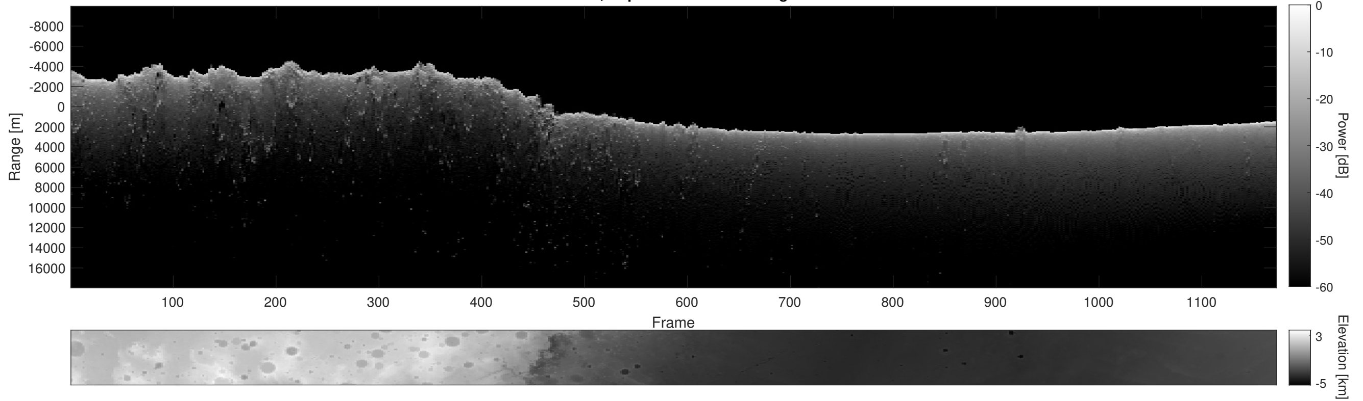
Orbit 6070, Depth-Corrected Cluttergram
