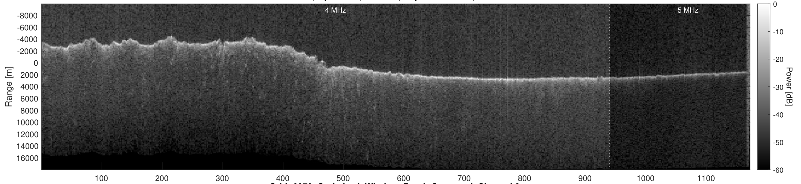
Orbit 6070, Optimized, Window, Depth-Corrected, Channel 2
