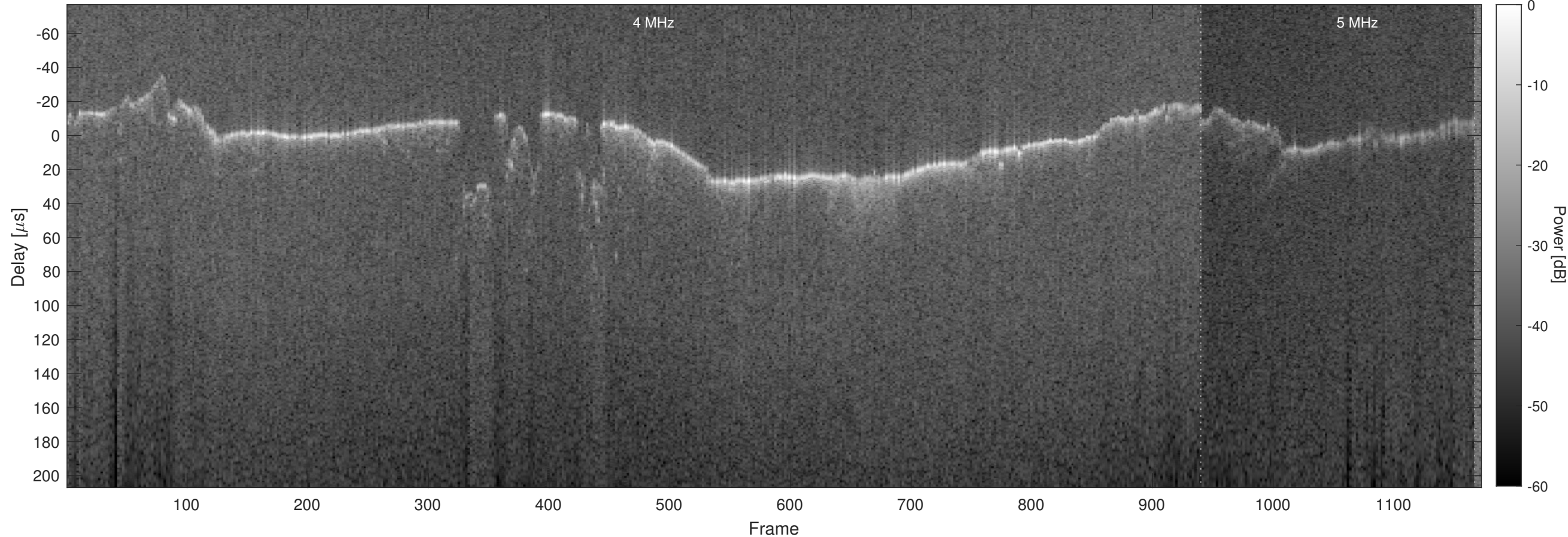
Orbit 6072, Chapman, No Window, Channel 2
