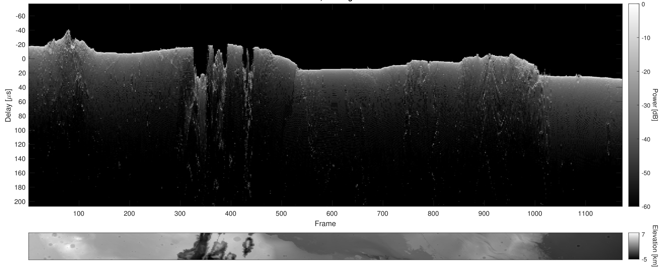
Orbit 6072, Cluttergram
