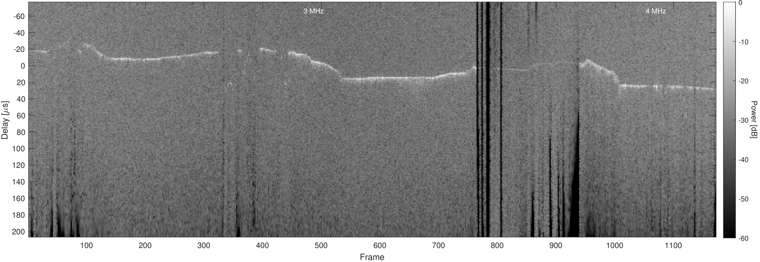
Orbit 6072, Optimized, No Window, Channel 2
