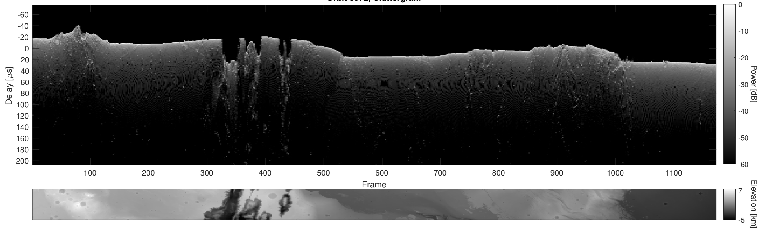
Orbit 6072, Cluttergram
