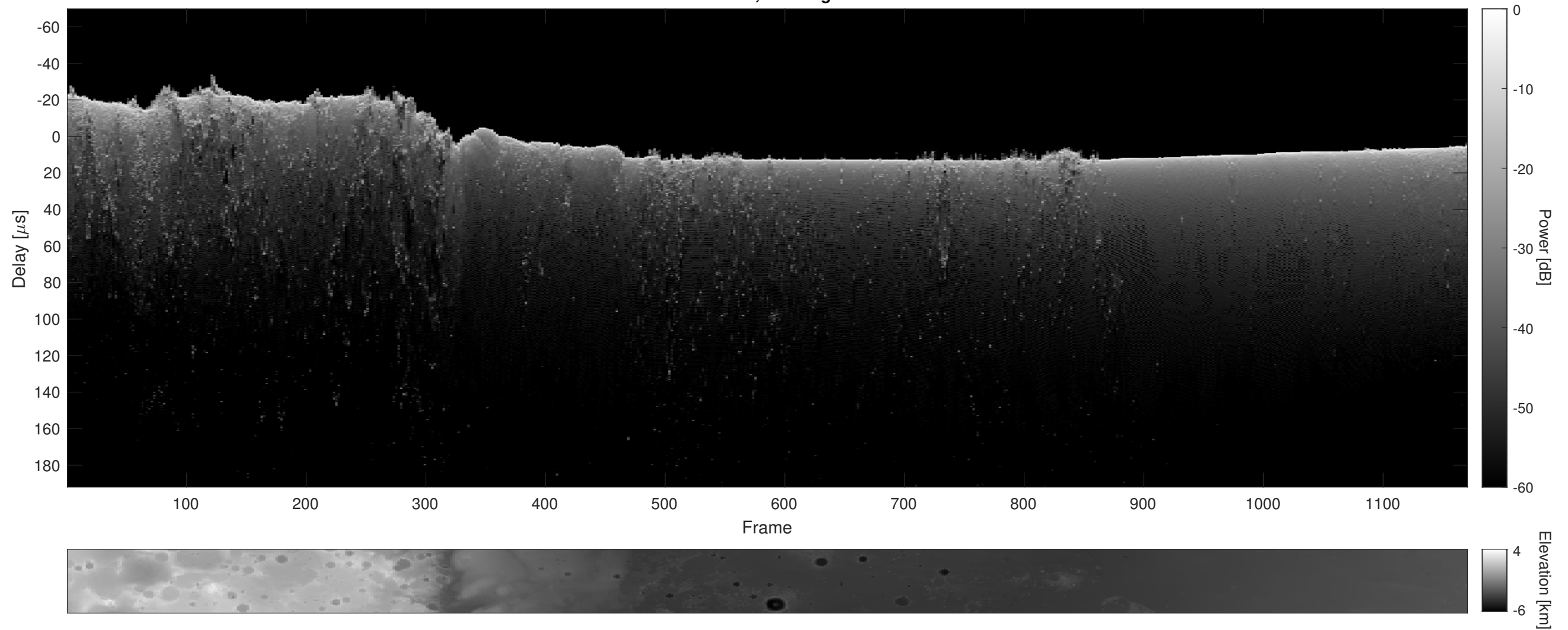
Orbit 6073, Cluttergram
