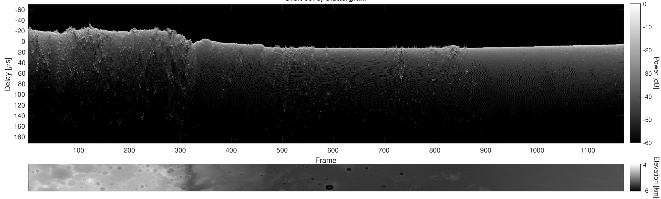
Orbit 6073, Cluttergram
