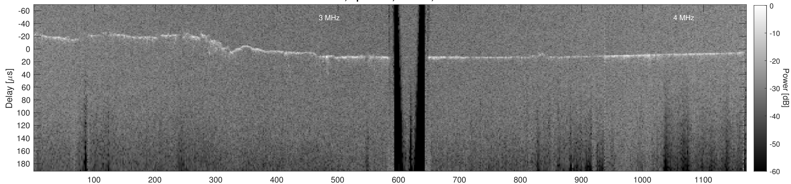
Orbit 6073, Cluttergram
