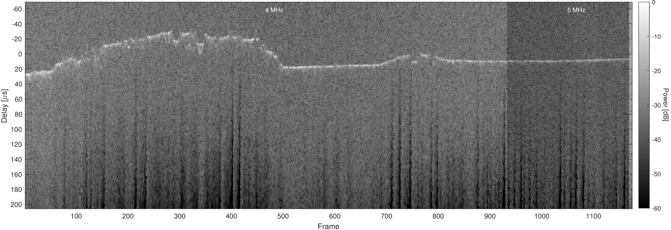
Orbit 6074, Optimized, Window, Channel 2
