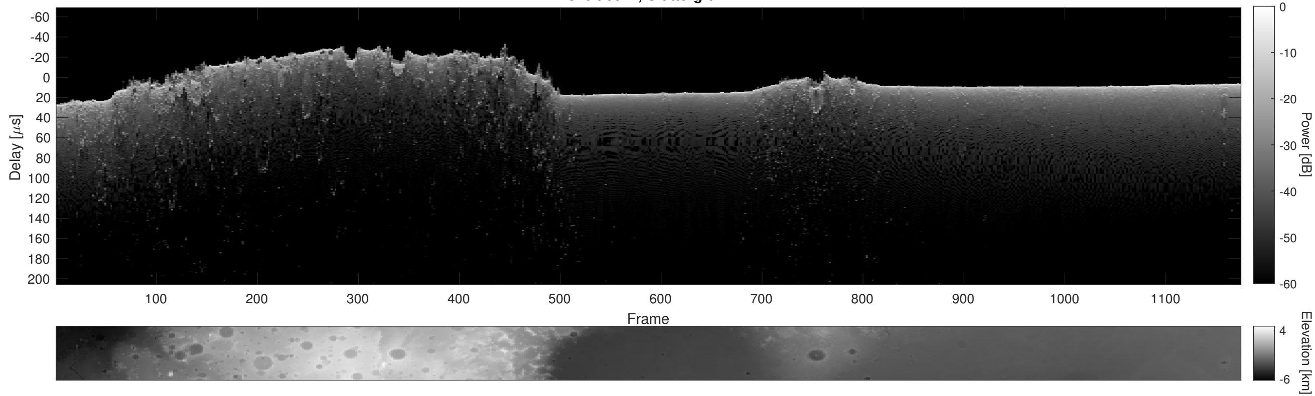
Orbit 6074, Cluttergram
