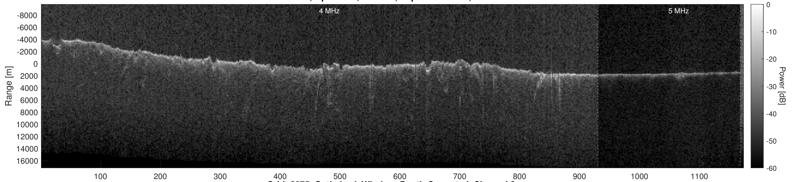
Orbit 6075, Optimized, Window, Depth-Corrected, Channel 2
