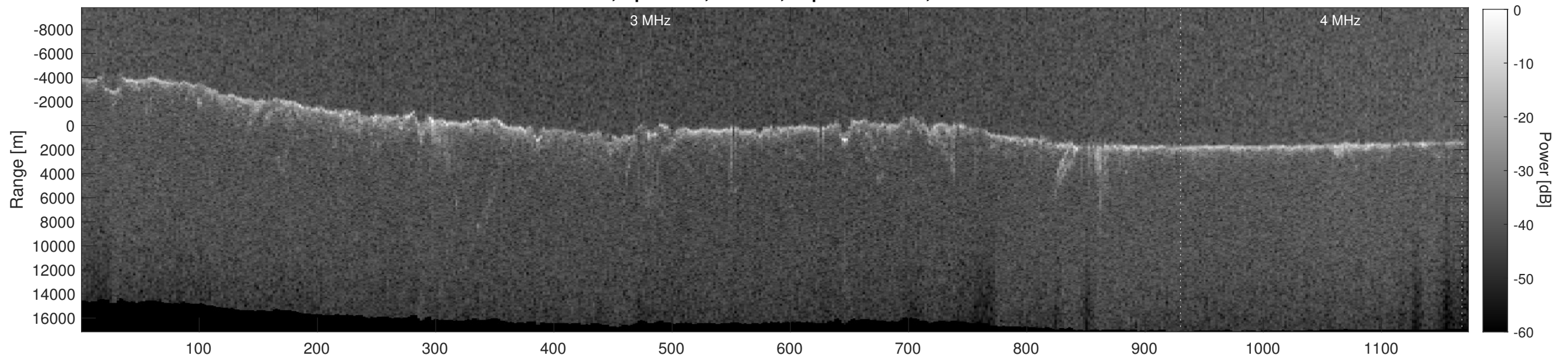
Orbit 6075, Depth-Corrected Cluttergram
