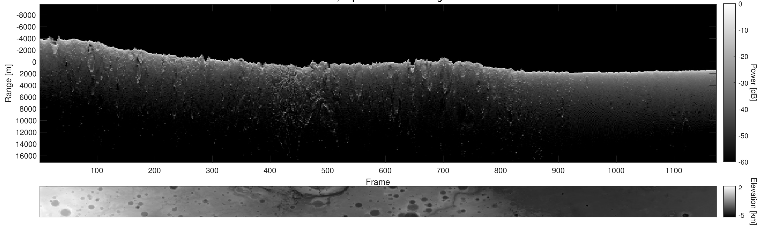
Orbit 6075, Depth-Corrected Cluttergram
