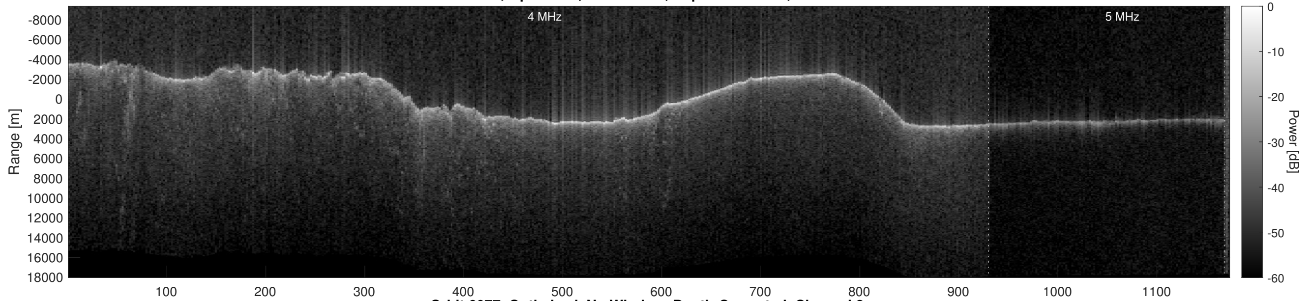
Orbit 6077, Optimized, No Window, Depth-Corrected, Channel 2
