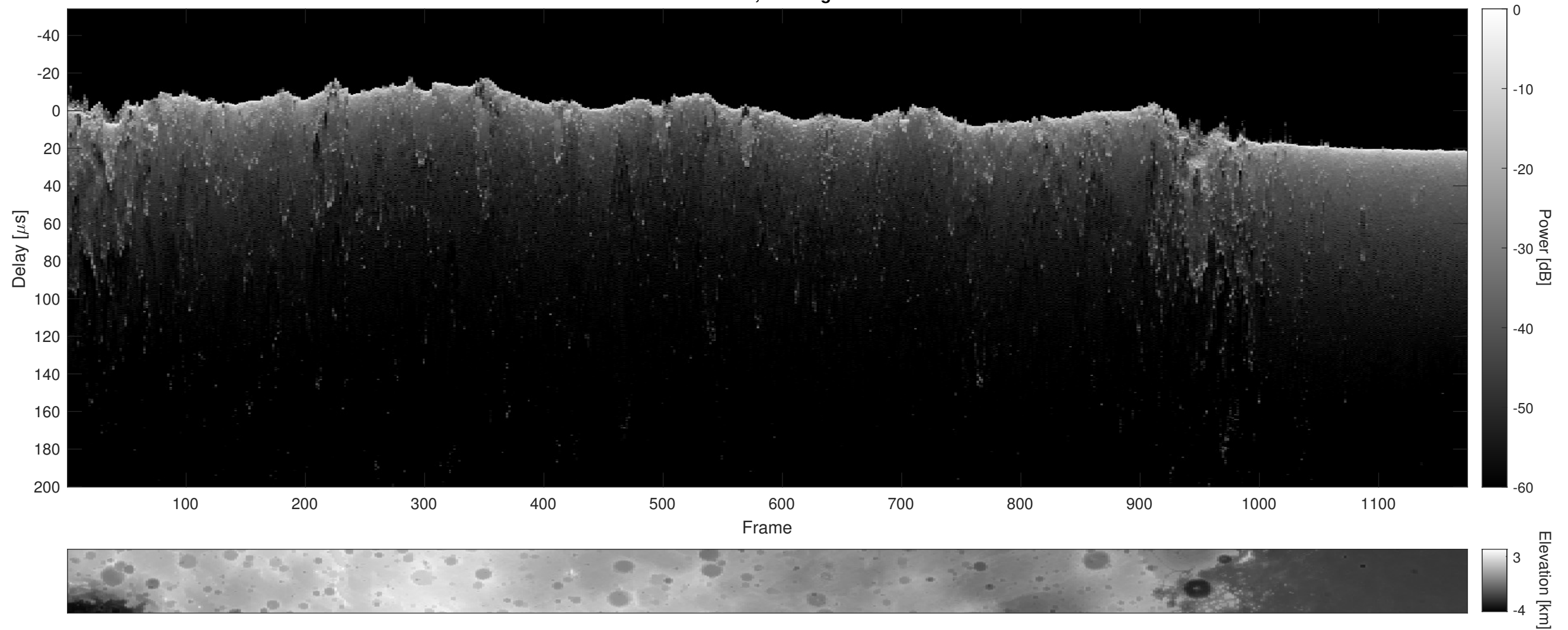
Orbit 6078, Cluttergram
