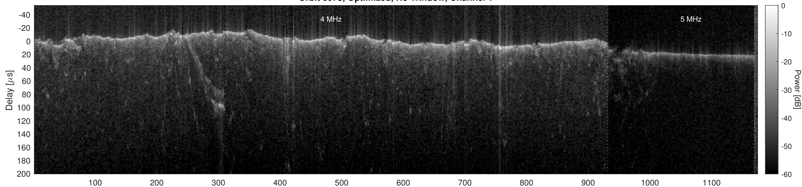
Orbit 6078, Optimized, No Window, Channel 2
