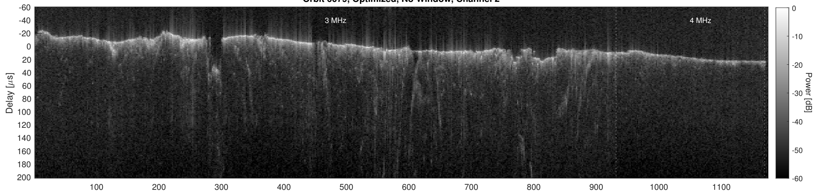
Orbit 6079, Cluttergram
