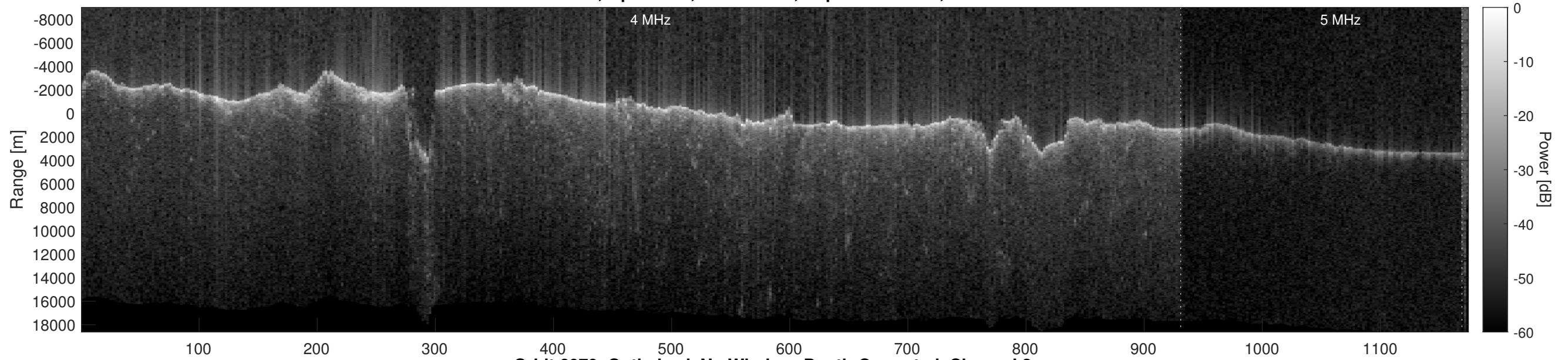
Orbit 6079, Optimized, No Window, Depth-Corrected, Channel 2
