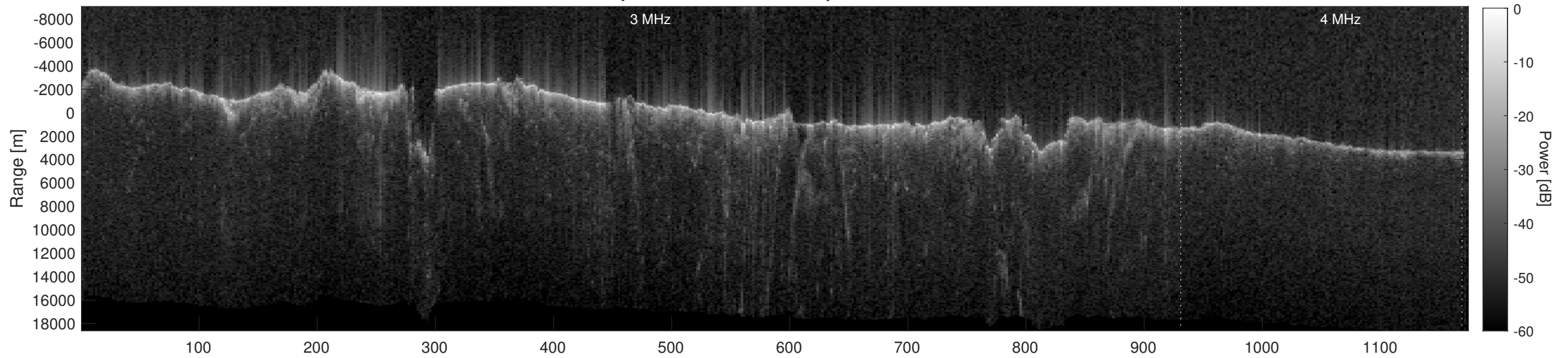
Orbit 6079, Depth-Corrected Cluttergram
