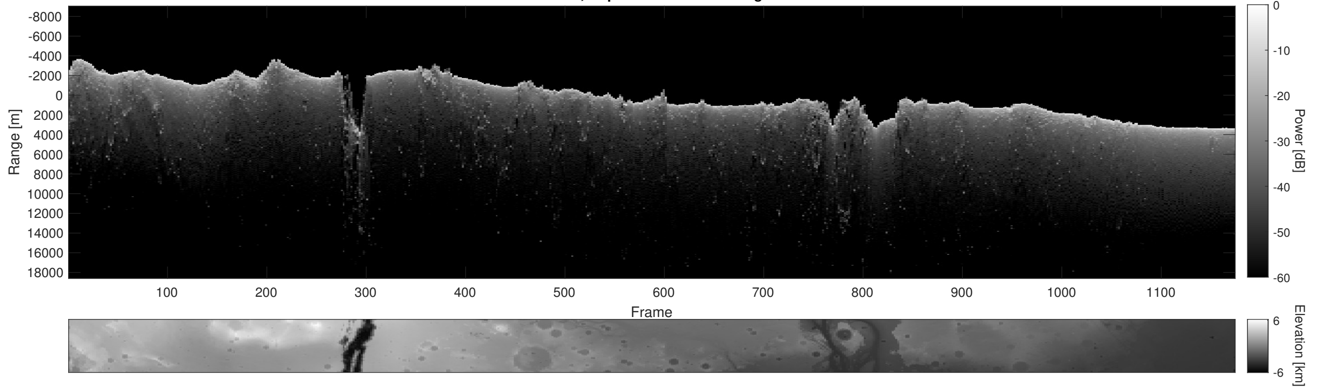
Orbit 6079, Depth-Corrected Cluttergram
