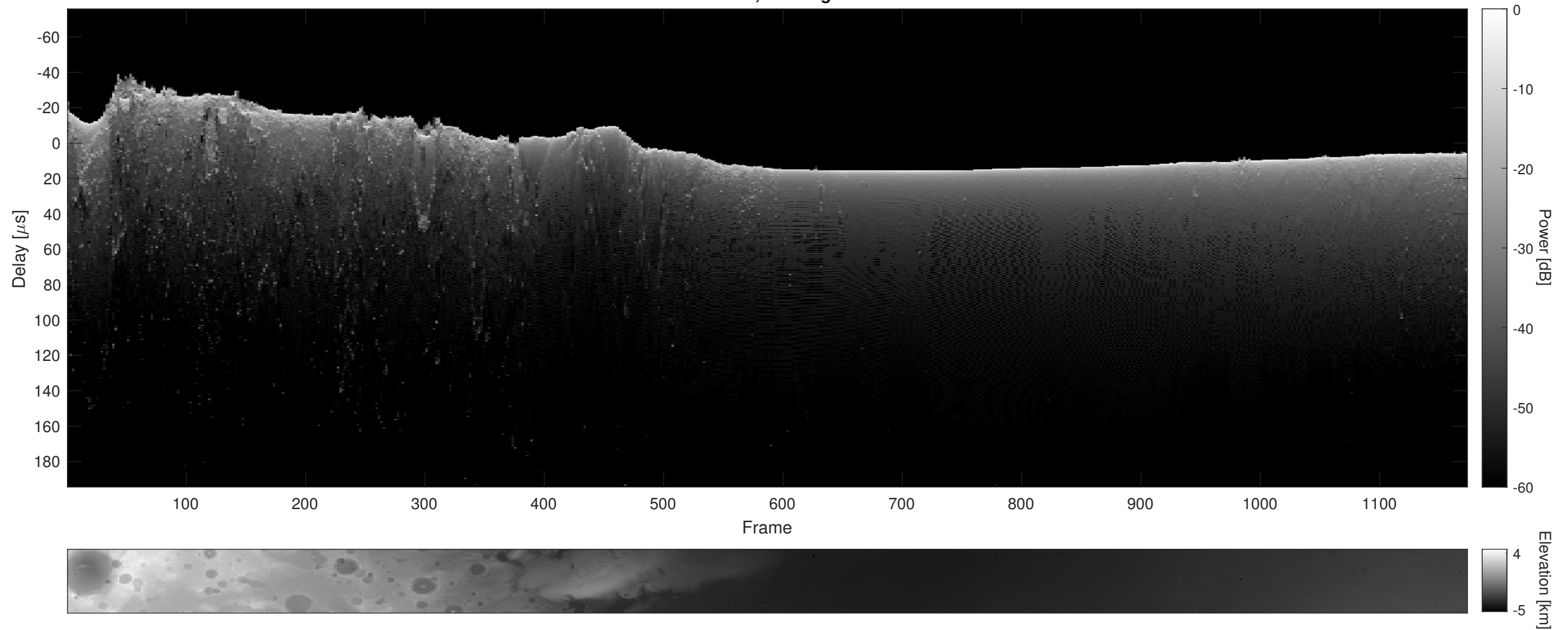
Orbit 6080, Cluttergram
