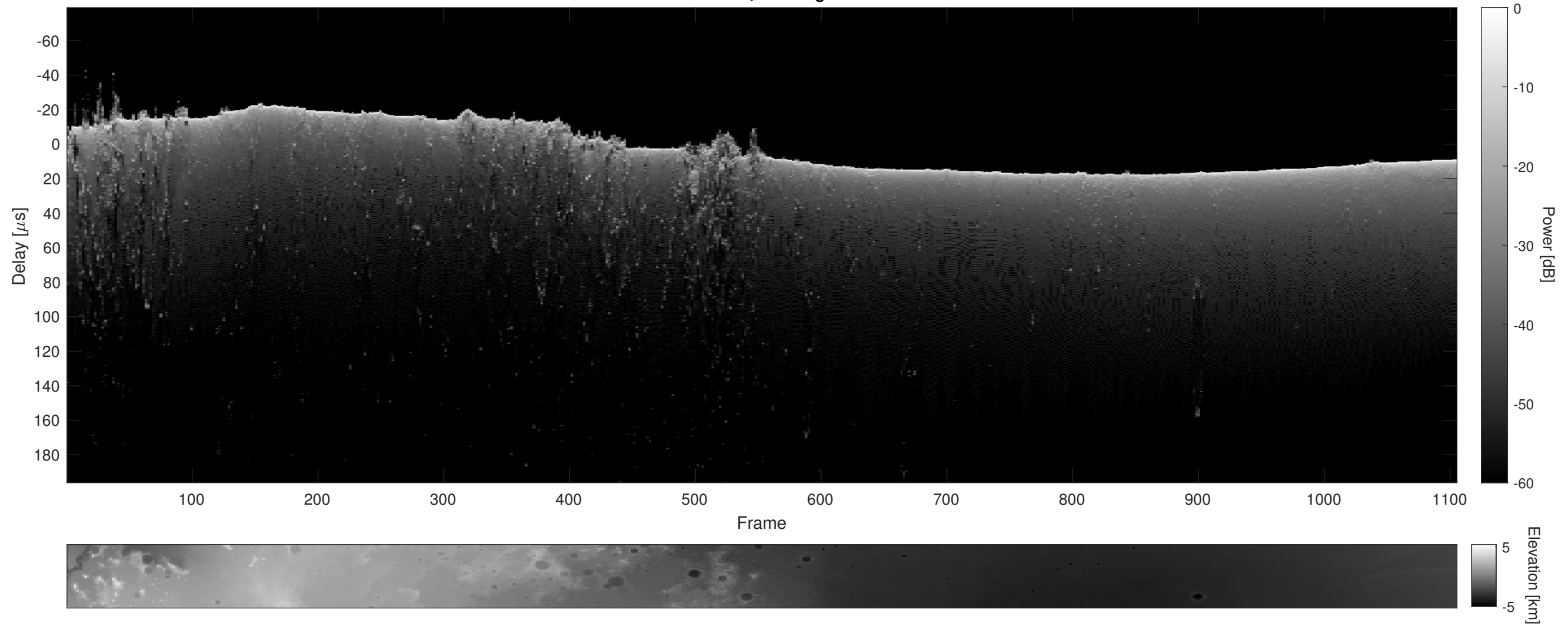
Orbit 6081, Cluttergram
