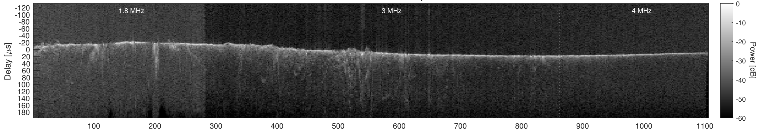
Orbit 6081, Cluttergram
