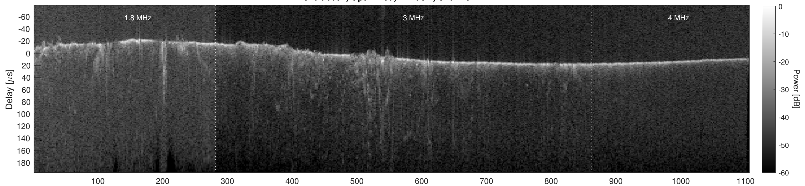
Orbit 6081, Cluttergram
