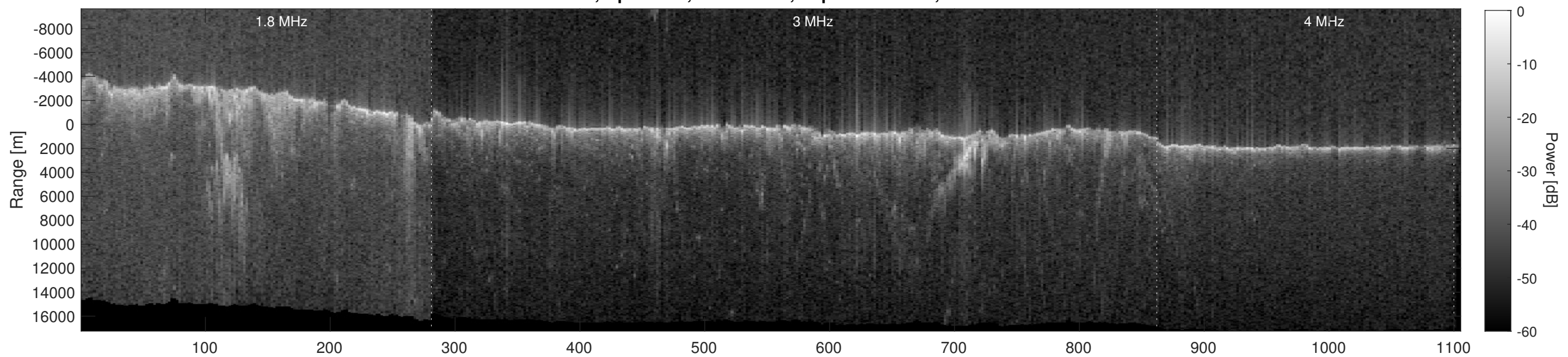
Orbit 6082, Depth-Corrected Cluttergram
