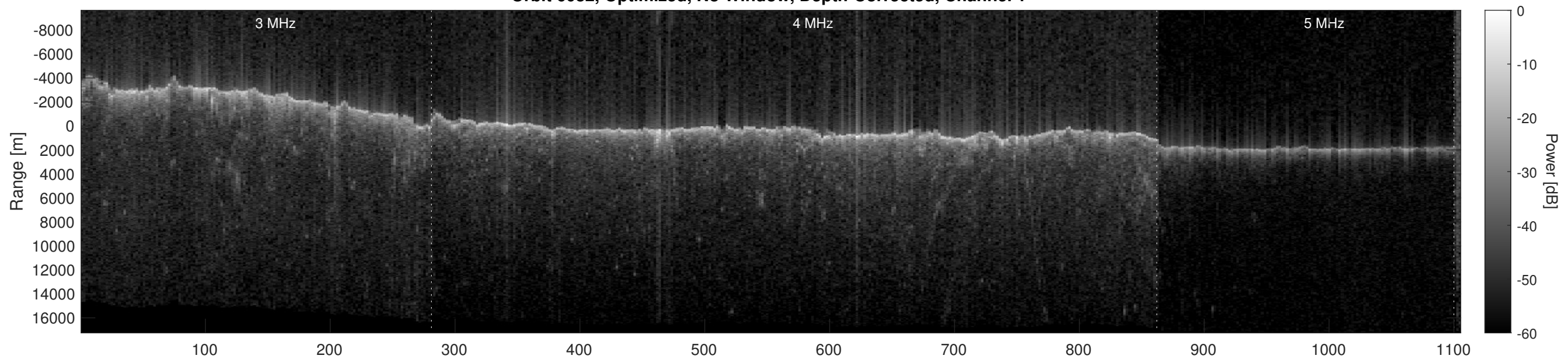
Orbit 6082, Optimized, No Window, Depth-Corrected, Channel 2
