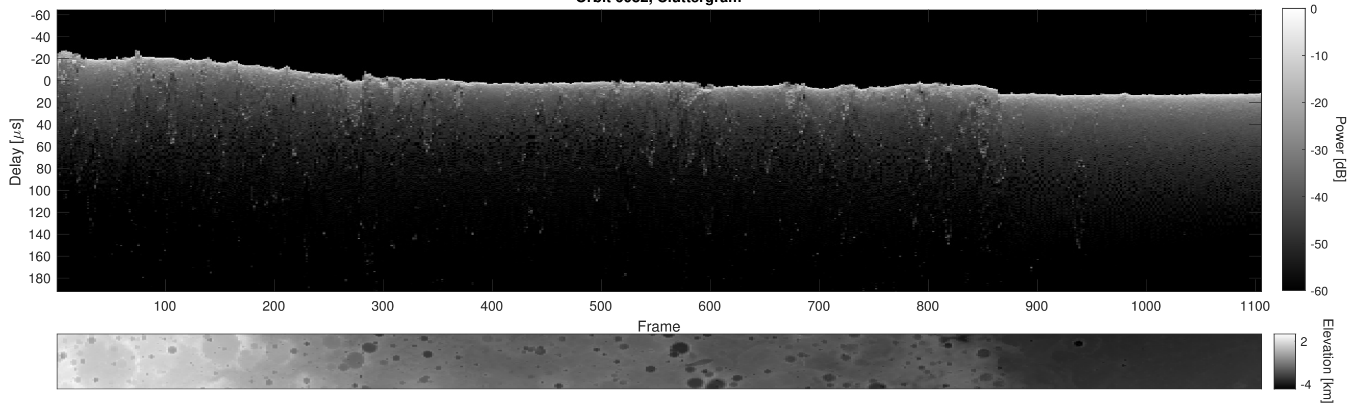
Orbit 6082, Cluttergram
