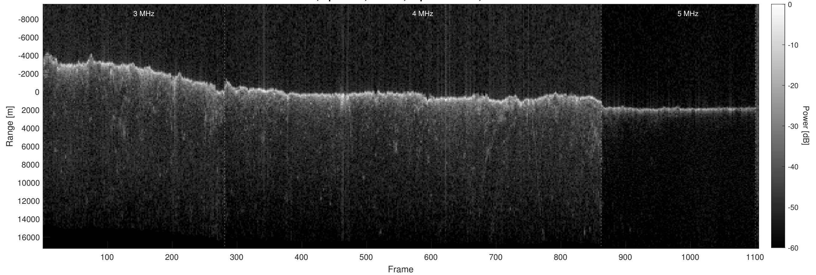
Orbit 6082, Optimized, Window, Depth-Corrected, Channel 2
