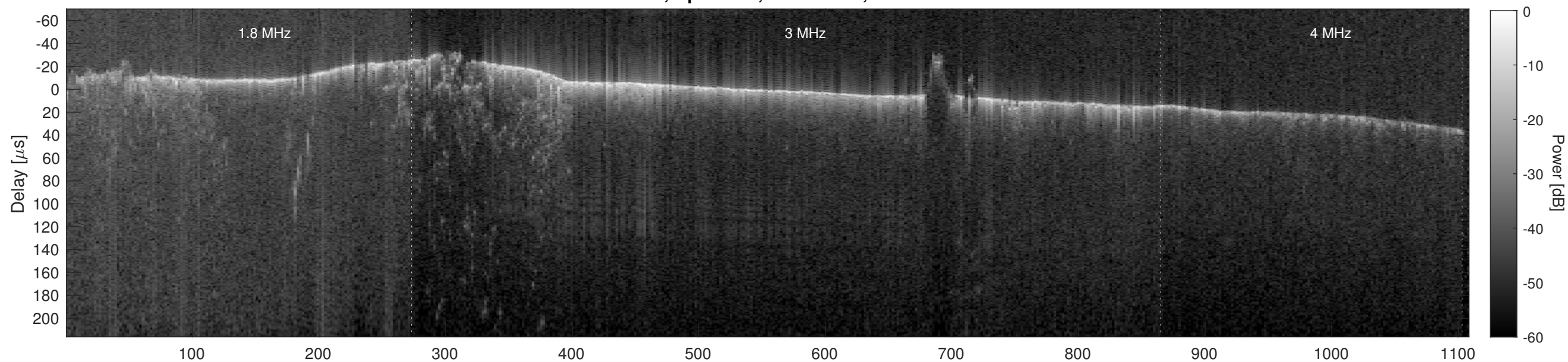
Orbit 6083, Cluttergram
