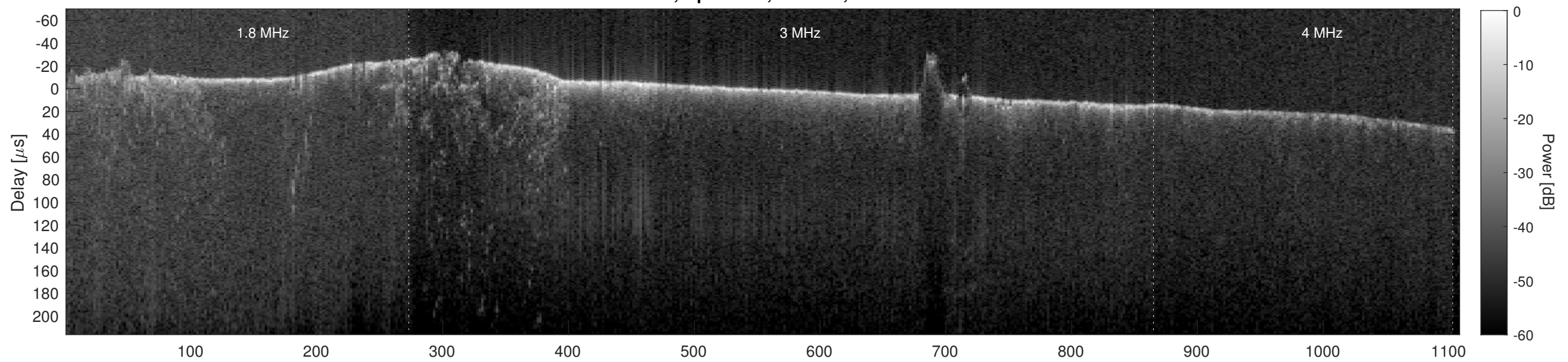
Orbit 6083, Cluttergram
