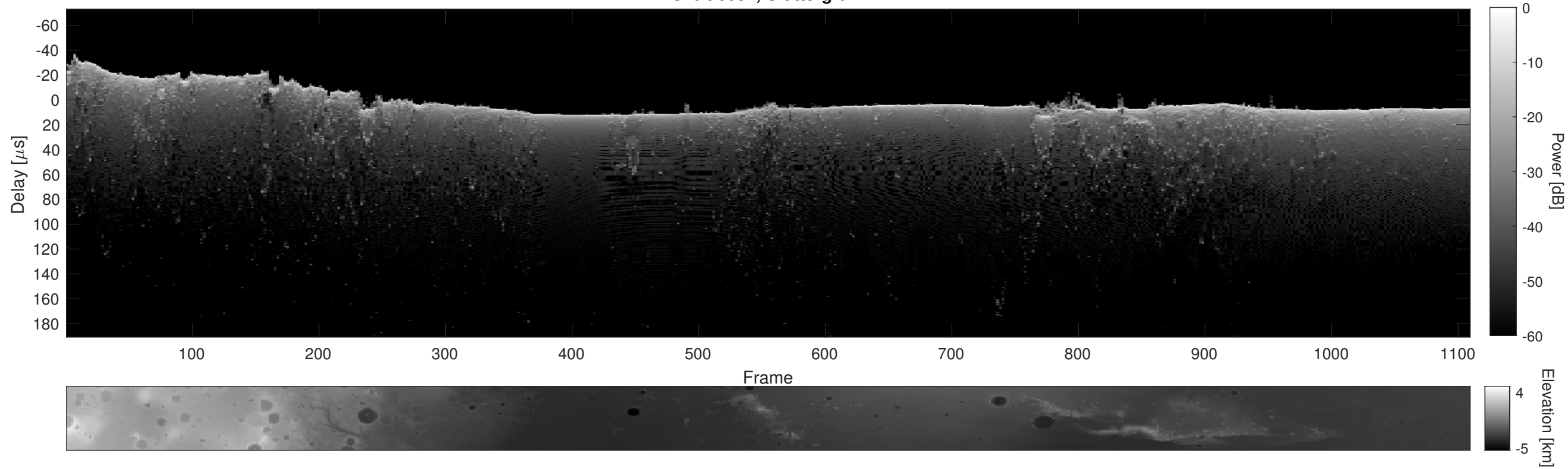
Orbit 6084, Cluttergram
