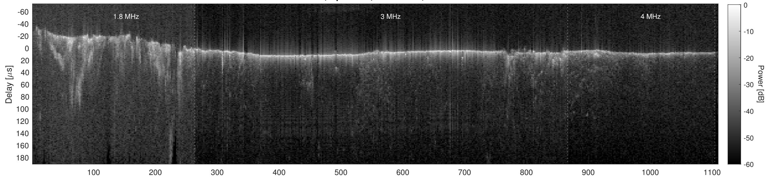
Orbit 6084, Cluttergram
