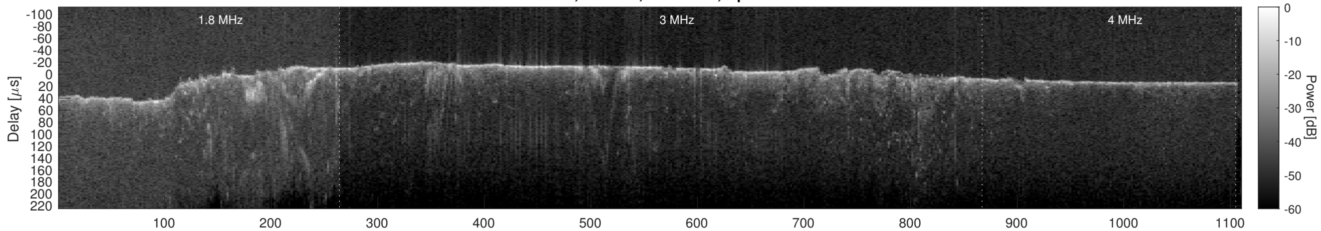
Orbit 6085, Cluttergram
