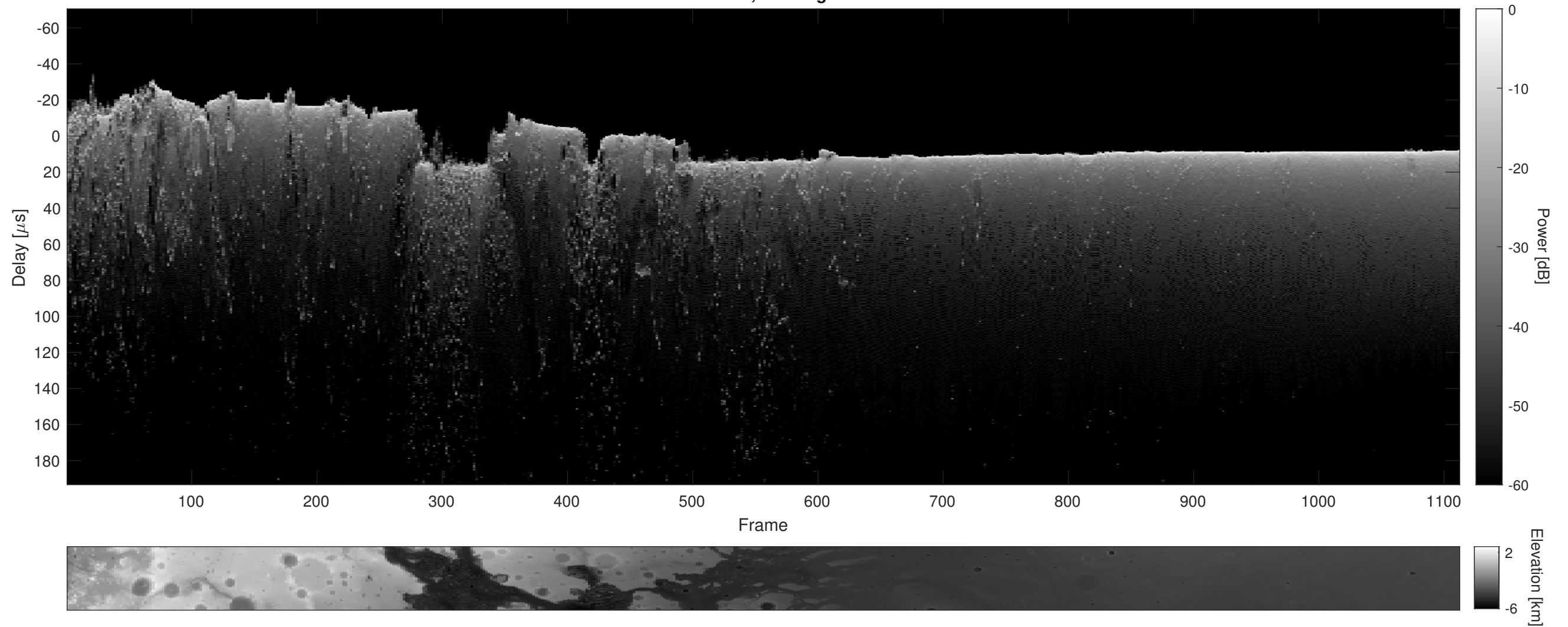
Orbit 6086, Cluttergram
