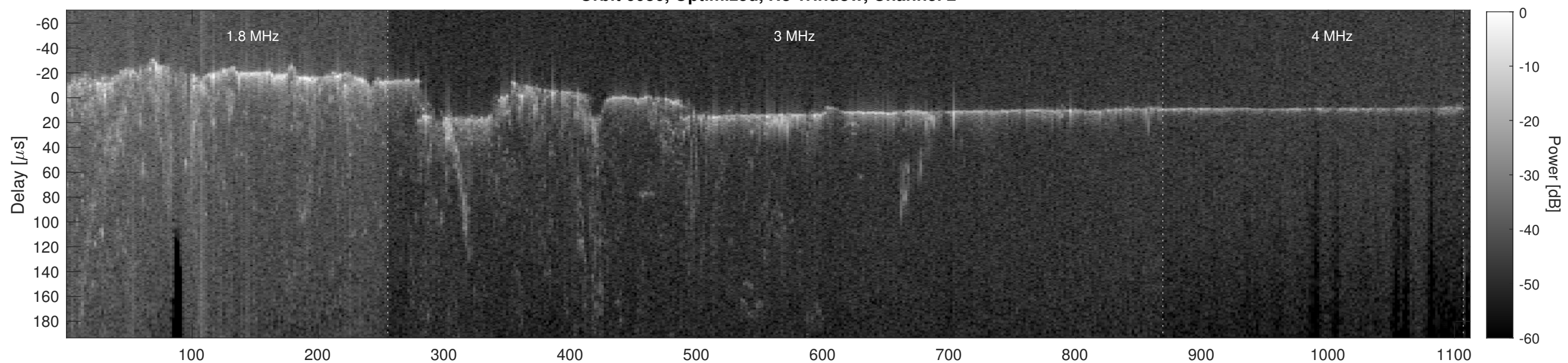
Orbit 6086, Cluttergram
