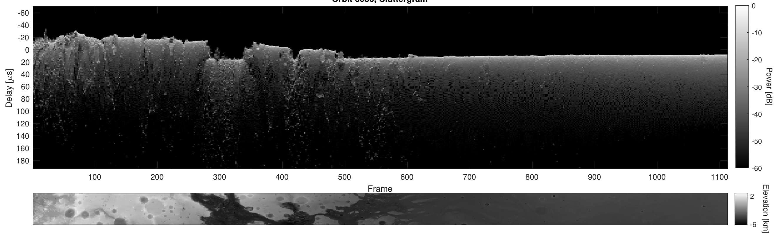
Orbit 6086, Cluttergram
