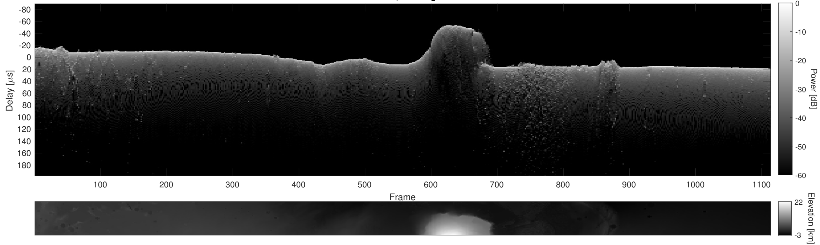
Orbit 6087, Cluttergram
