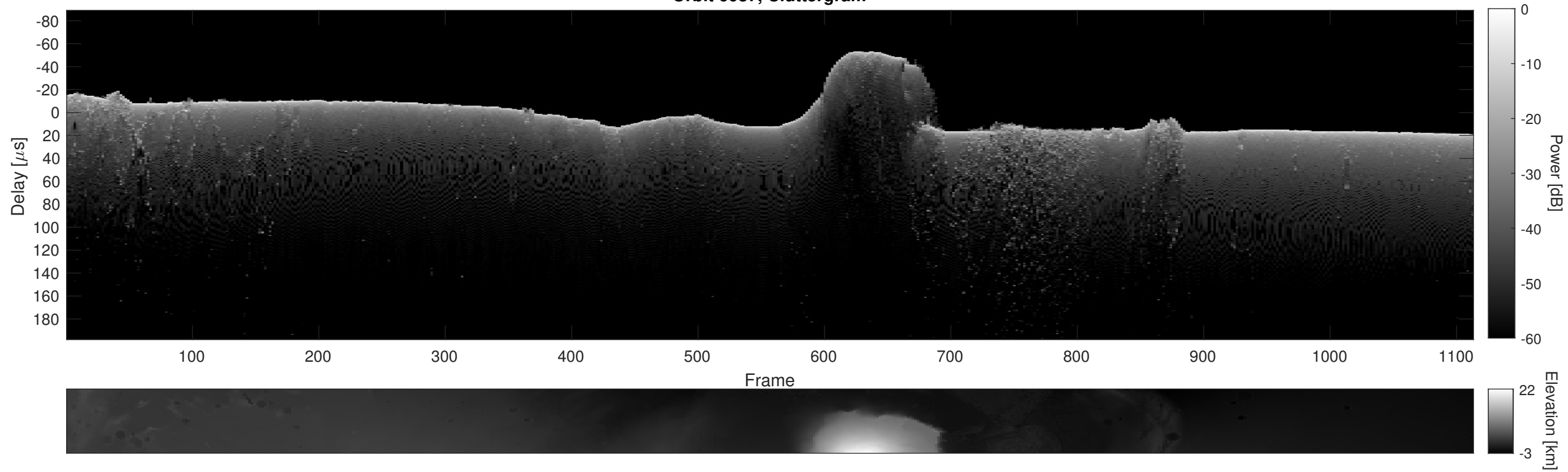
Orbit 6087, Cluttergram
