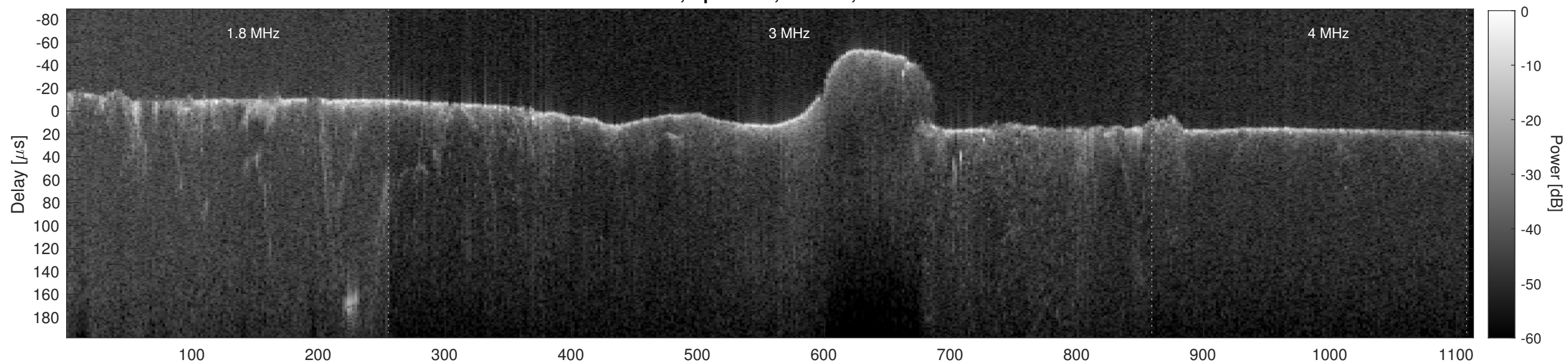
Orbit 6087, Cluttergram
