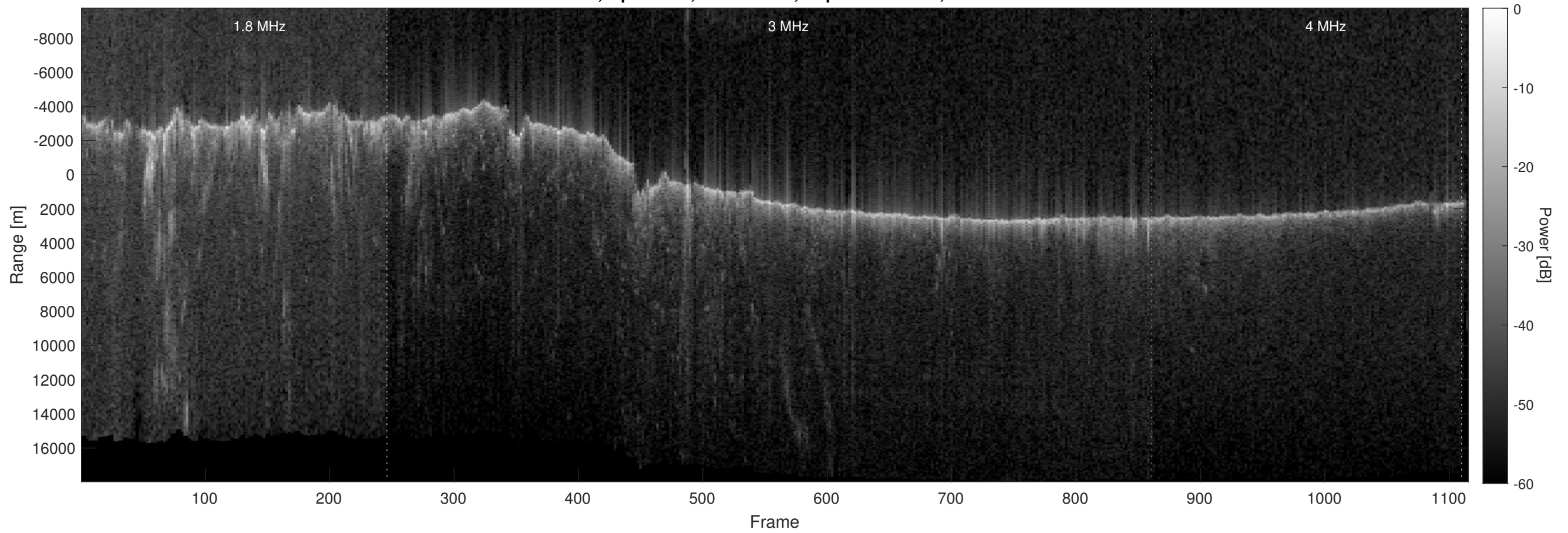
Orbit 6088, Optimized, No Window, Depth-Corrected, Channel 2
