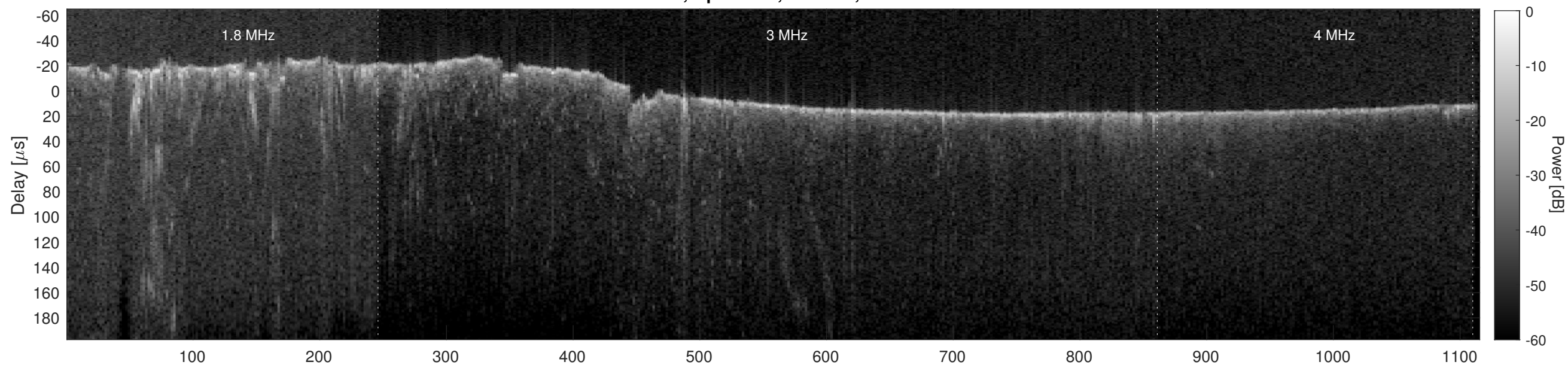
Orbit 6088, Cluttergram
