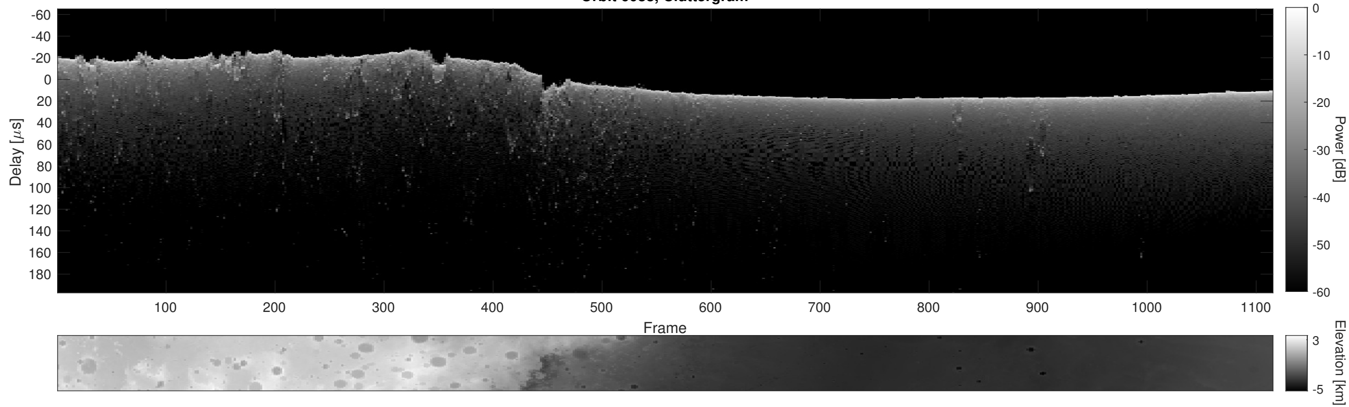
Orbit 6088, Cluttergram
