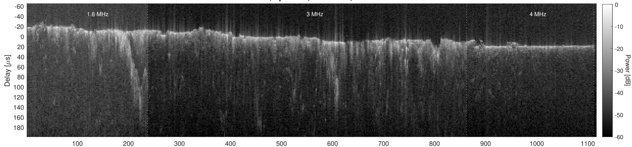
Orbit 6089, Cluttergram
