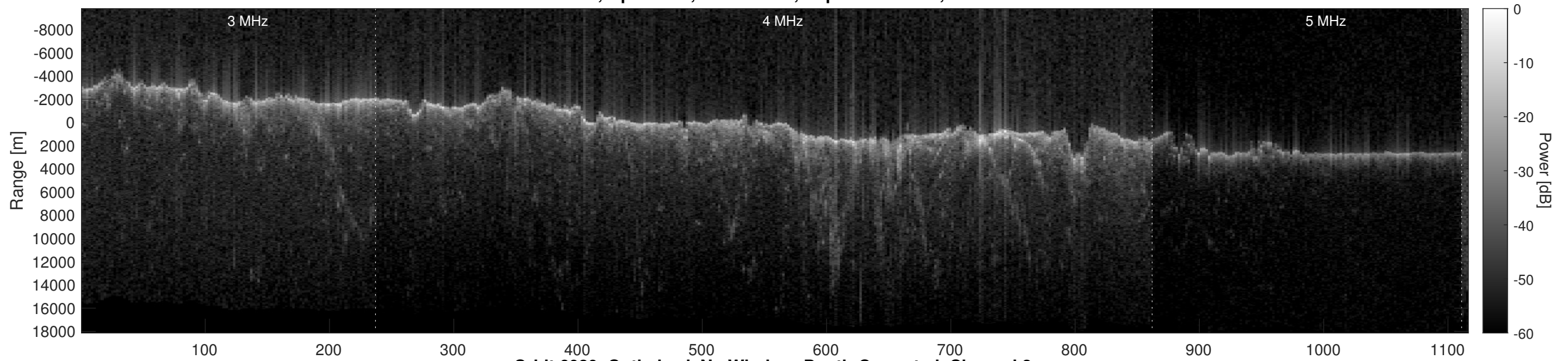
Orbit 6089, Optimized, No Window, Depth-Corrected, Channel 2
