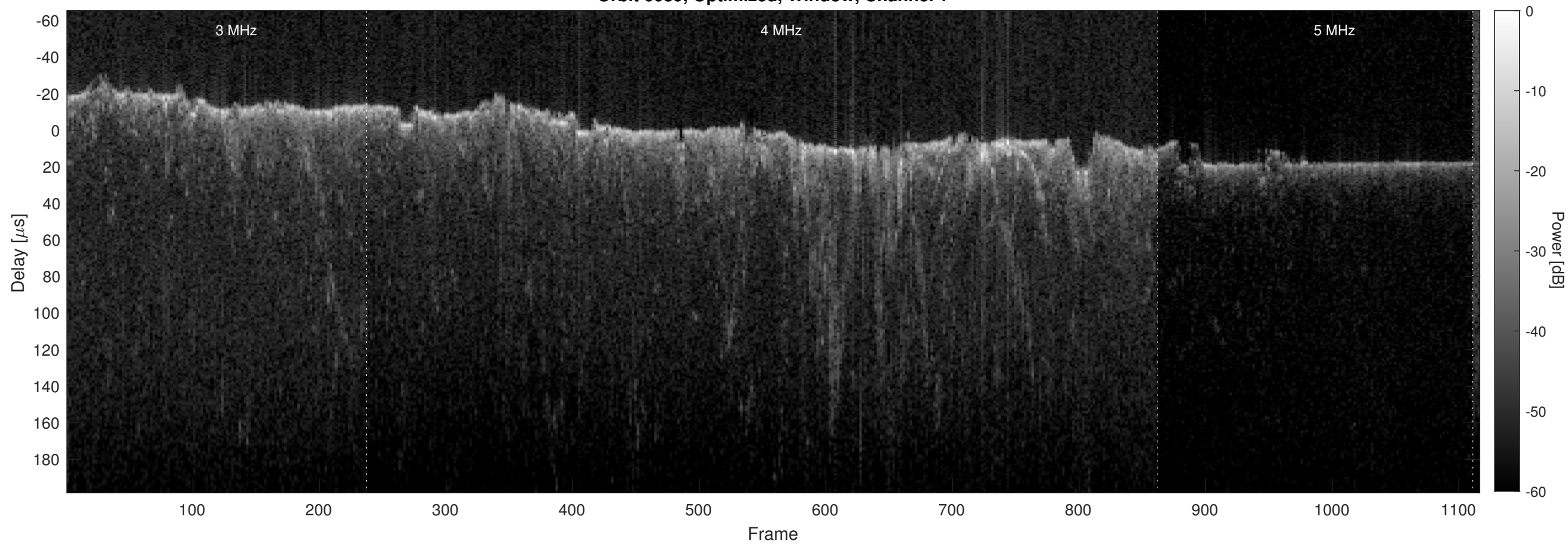
Orbit 6089, Optimized, Window, Channel 2
