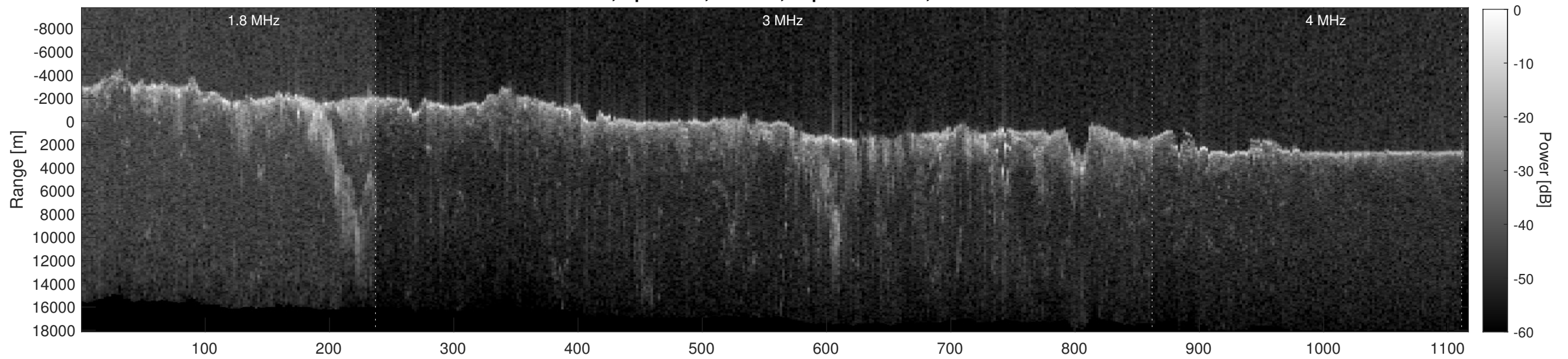
Orbit 6089, Depth-Corrected Cluttergram
