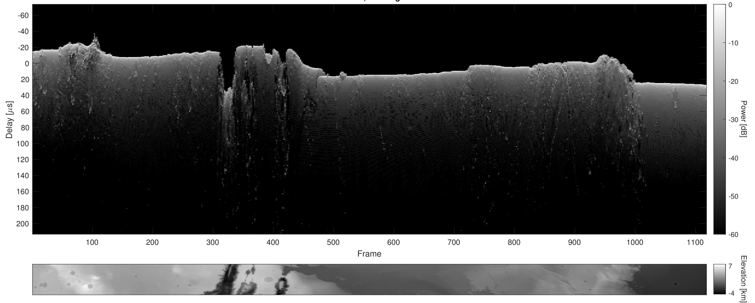
Orbit 6090, Cluttergram
