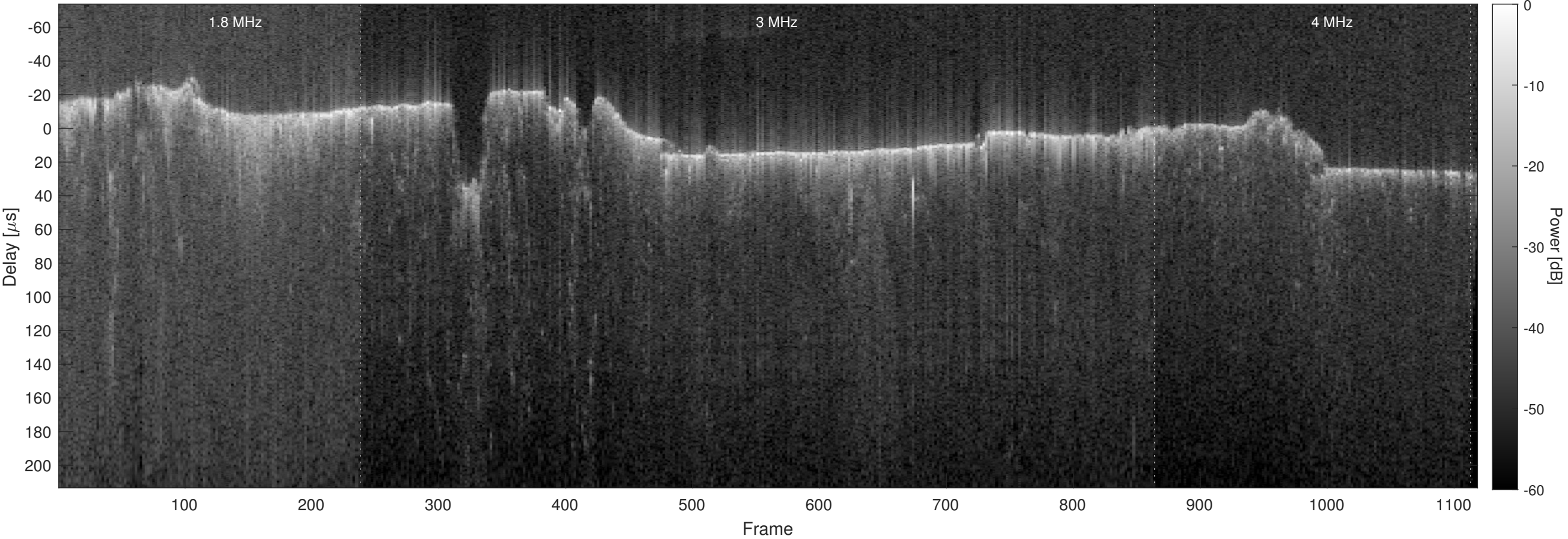
Orbit 6090, Optimized, No Window, Channel 2
