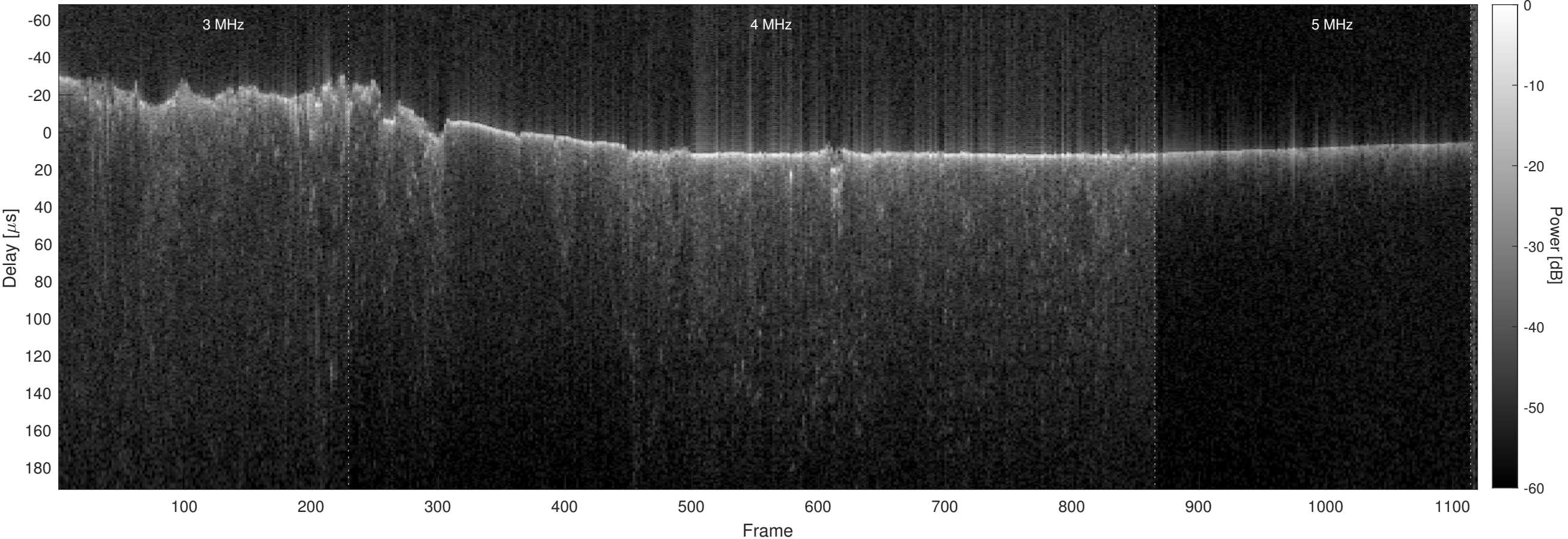
Orbit 6091, Optimized, No Window, Channel 2
