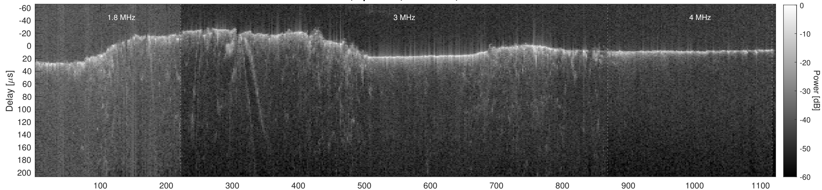
Orbit 6092, Cluttergram
