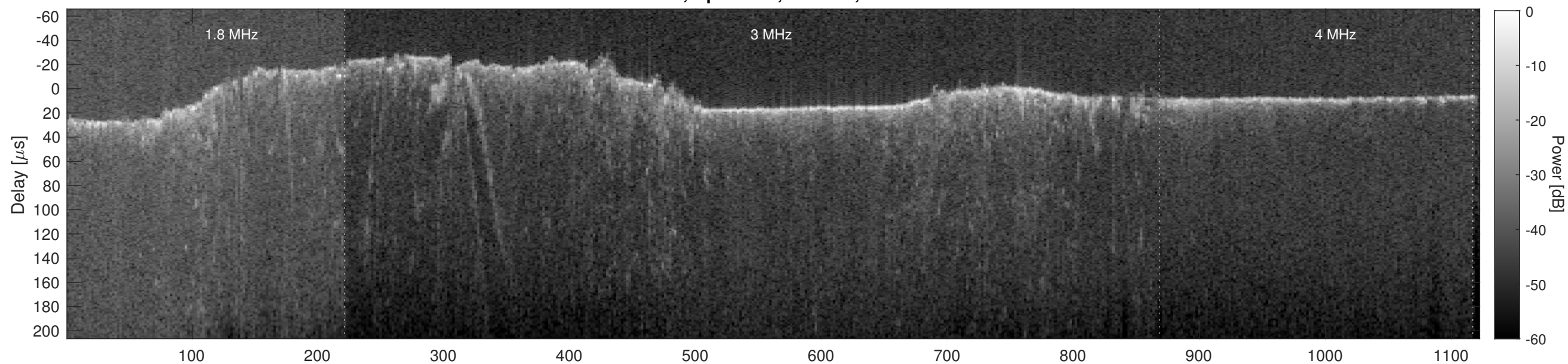
Orbit 6092, Cluttergram
