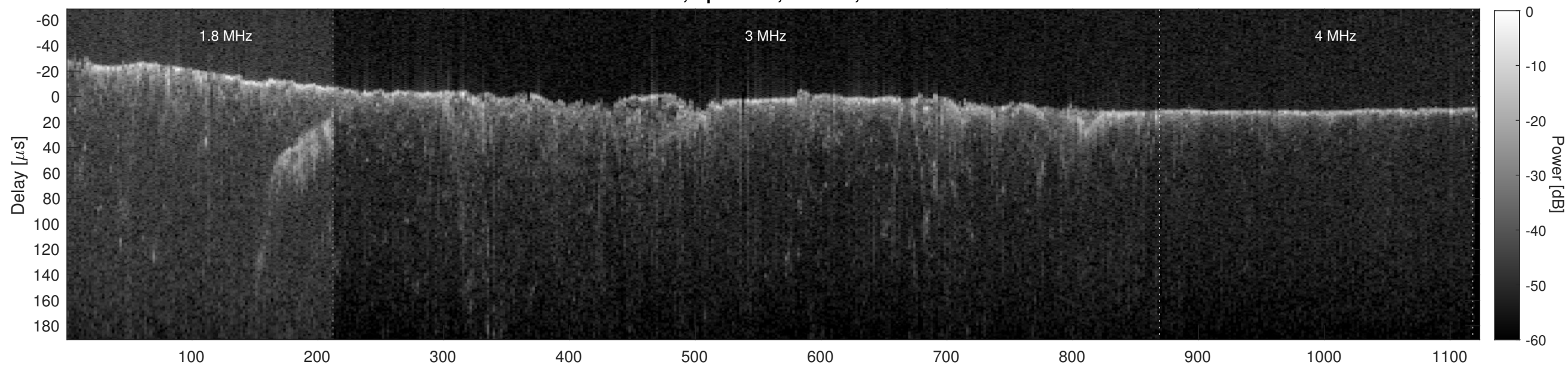
Orbit 6093, Cluttergram
