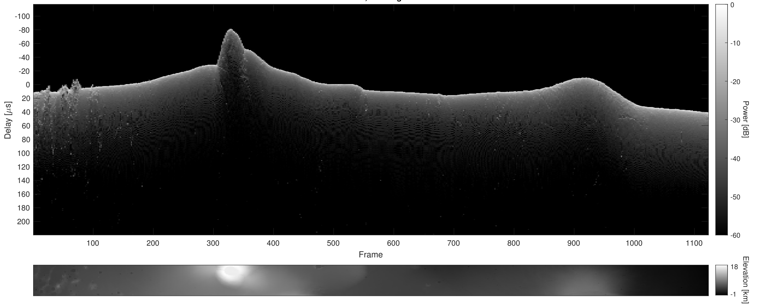
Orbit 6094, Cluttergram
