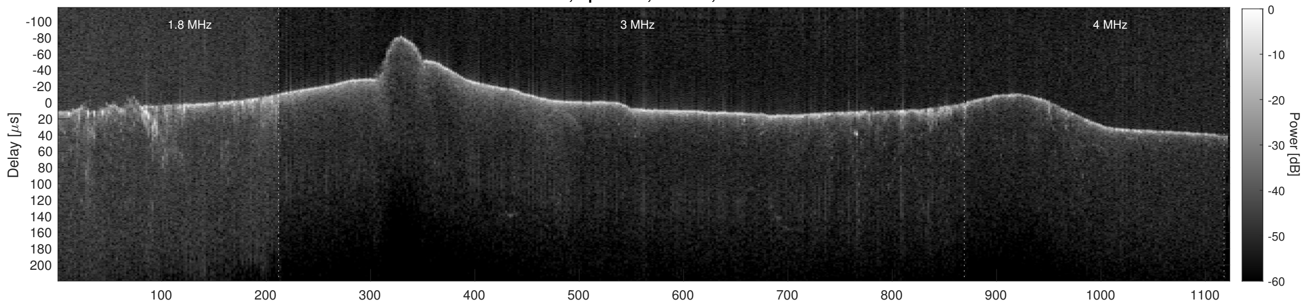
Orbit 6094, Cluttergram
