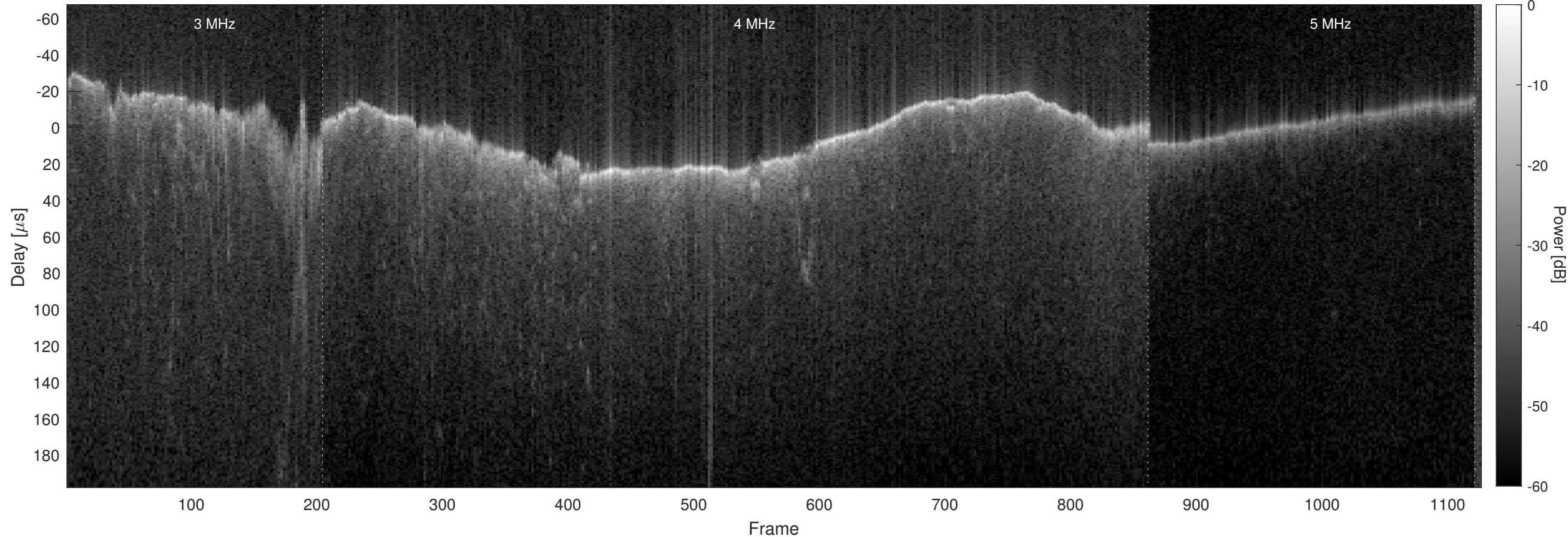
Orbit 6095, Chapman, No Window, Channel 2
