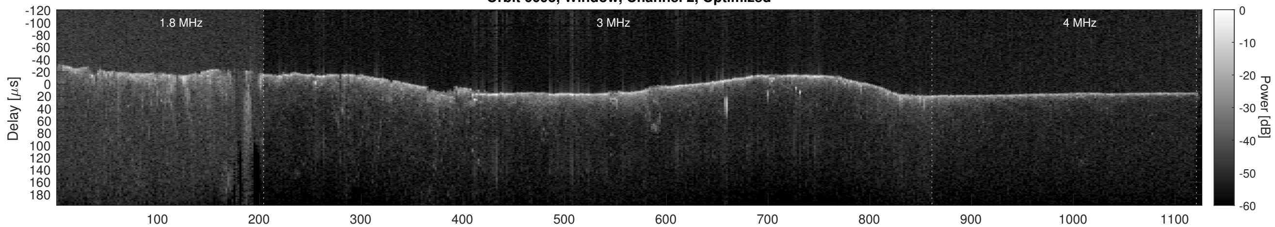
Orbit 6095, Cluttergram
