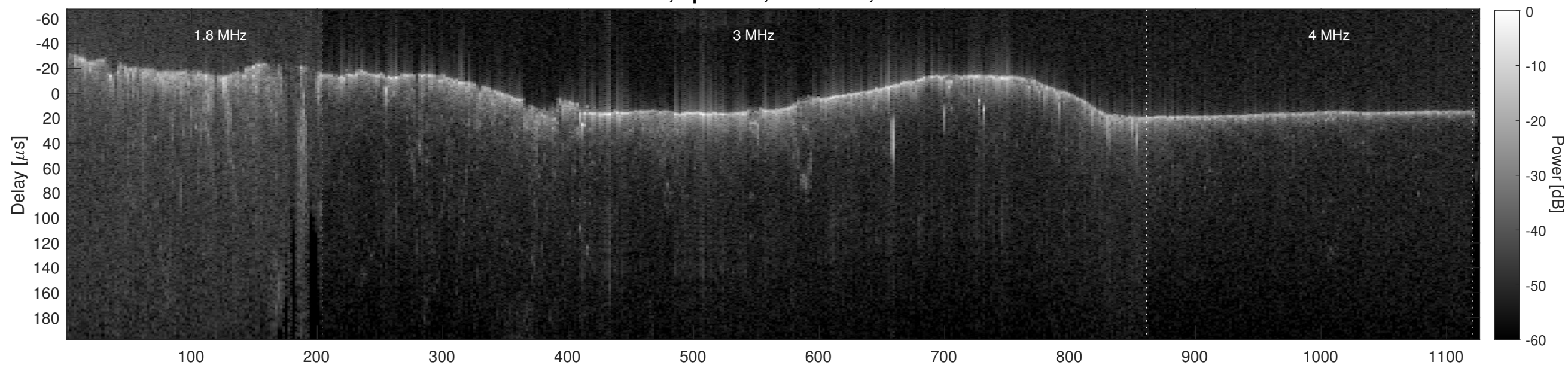
Orbit 6095, Cluttergram
