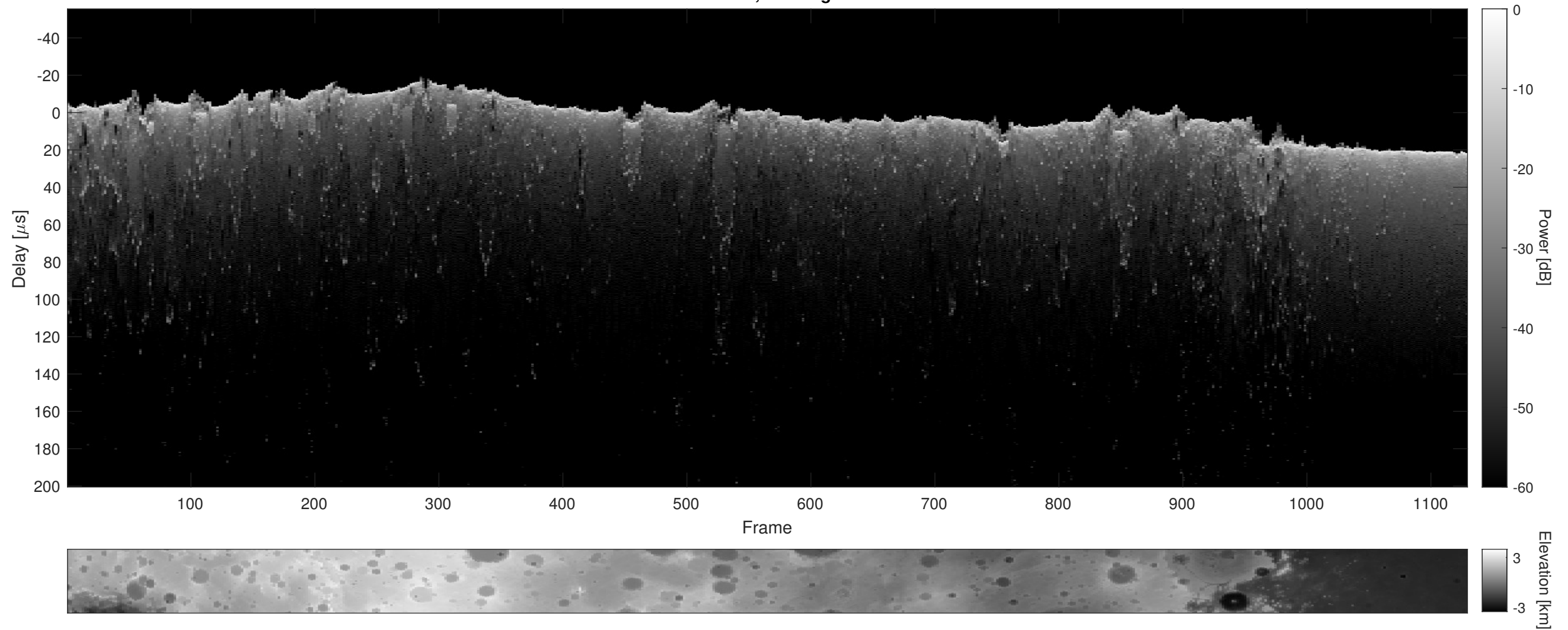
Orbit 6096, Cluttergram
