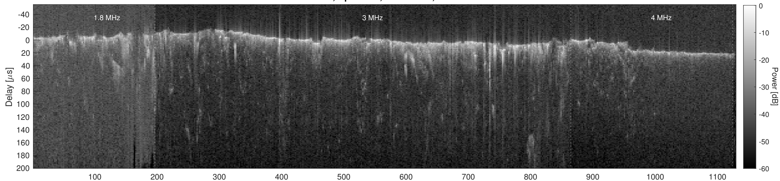
Orbit 6096, Cluttergram
